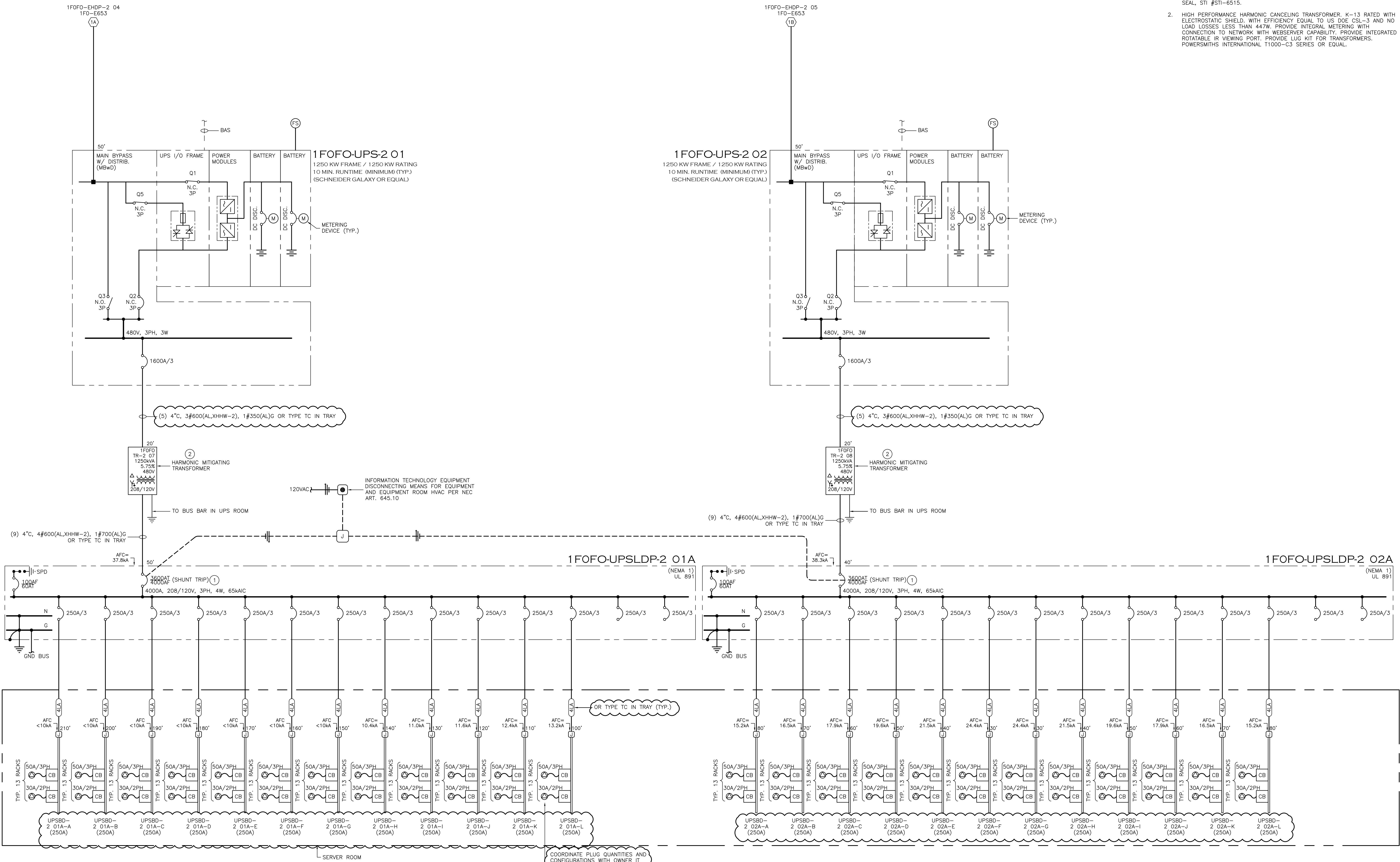
1 ONE LINE DIAGRAM - DATA CENTER UPS ROOM 1 NO SCALE
